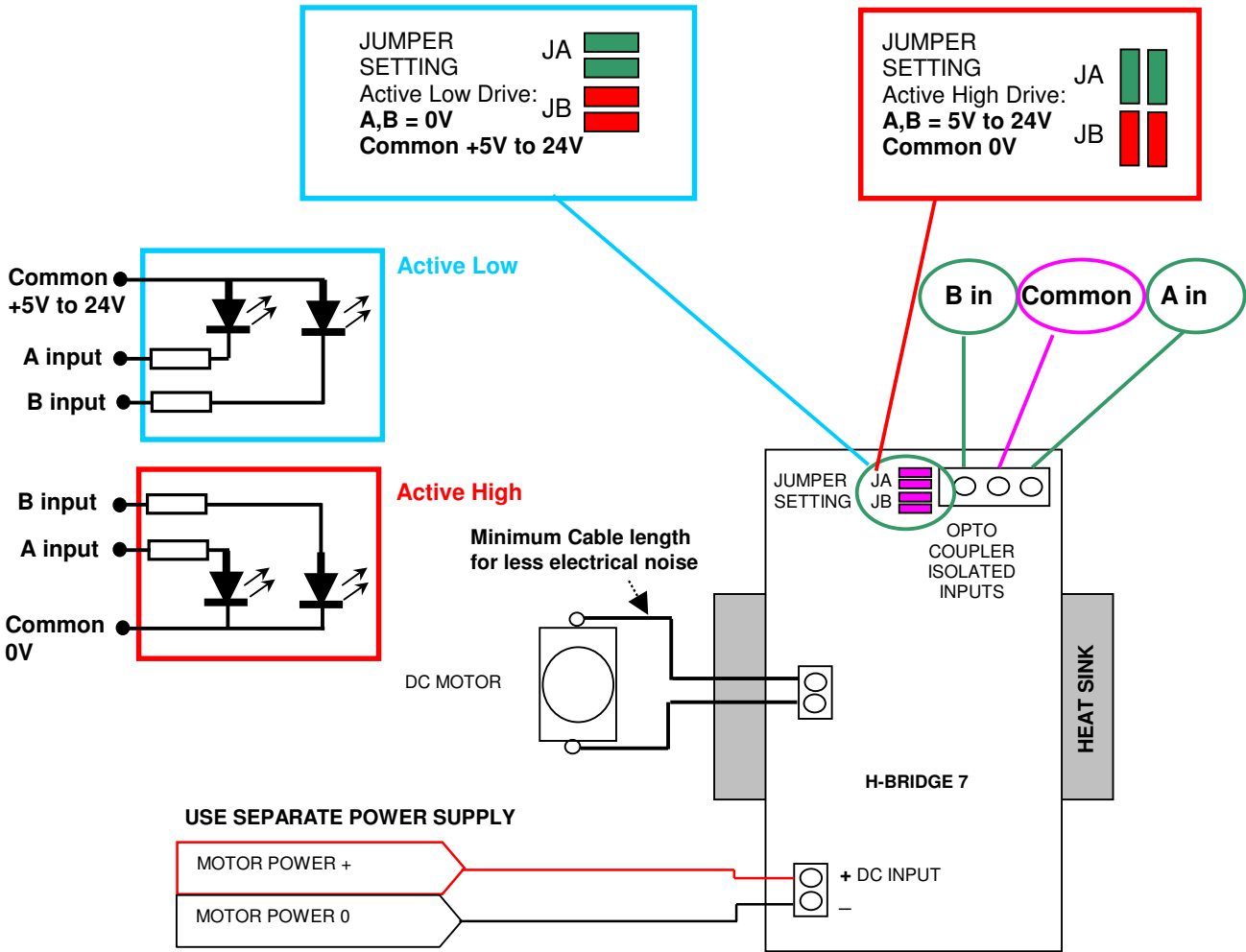
Wiring diagram with H-Bridge7
